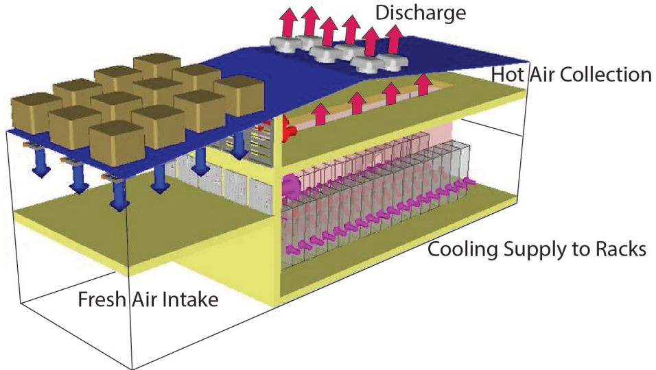
Figure 4.5: Airflow schematic of an air-economized datacenter (source: Perspectives, James Hamilton's blog).
