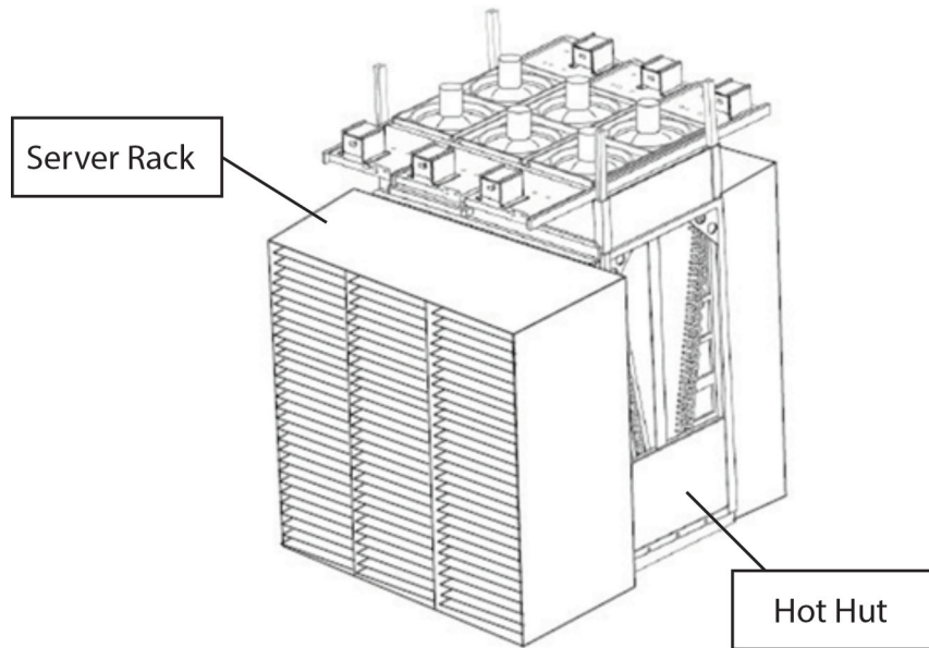
Figure 4.13: Racks are placed against the “Hot Hut” creating a warm air capture plenum.
