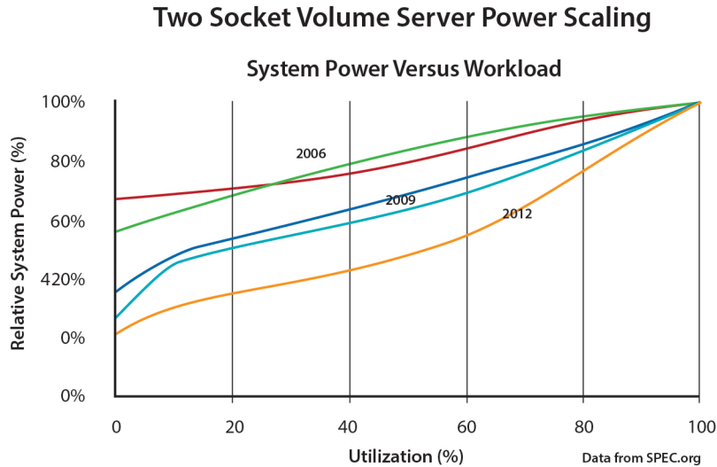
Figure 5.7: Normalized system power vs. utilization in Intel servers from 2006 and 2012 (Courtesy of Winston Saunders, Intel). The green and red lines represent 2006 servers, the two blue ones are 2009 servers, and the orange line is a more recent server. The chart indicates that Intel servers have become more energy proportional in that seven-year period.
