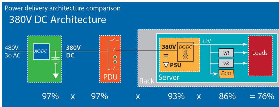
Figure 4.2: Traditional AC vs. DC distribution efficiency (Source: Pratt, Kumar, Bross, Aldridge, “Powering Compute Platforms in High Efficiency Data Centers,” IBM Technology Symposium, 2006).
