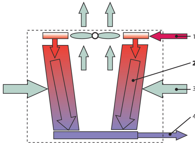
Figure 4.9: How a cooling tower works:
